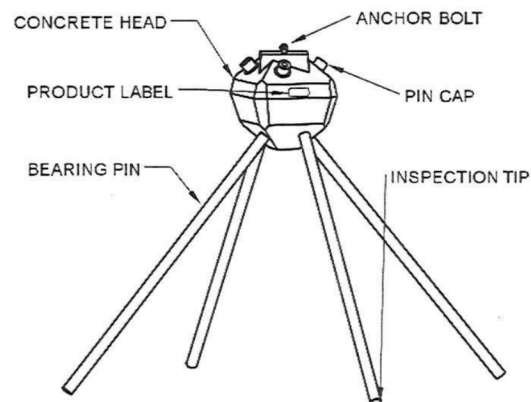
DIAMOND PIER FOUNDATION COMPONENTS
