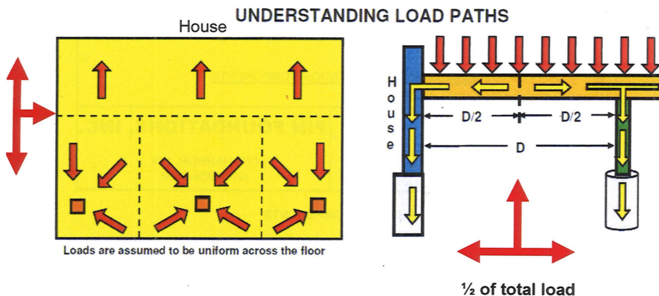
FIGURE 1: PLAN DIAGRAM
